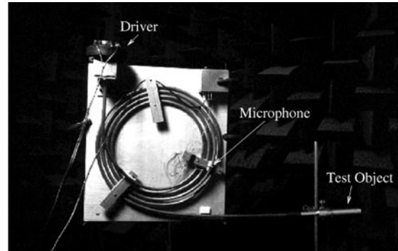
Figure 3. The pulse reflectometer.
