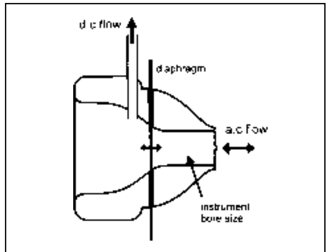
Figure 4. Mouthpiece with with enlarged throat.
