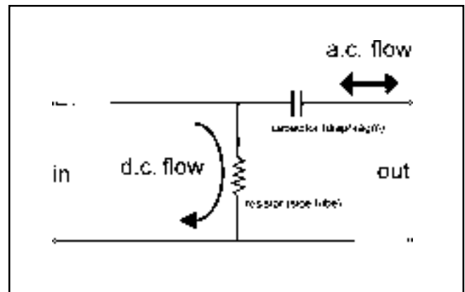
Figure 2. A.C. coupling for an electrical circuit and its similarity to a modified mouthpiece.
