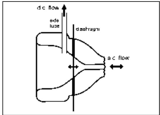
Figure 3. Modified mouthpiece with a diaphragm across the bore and a ‘throat’ through the side of the cup.
