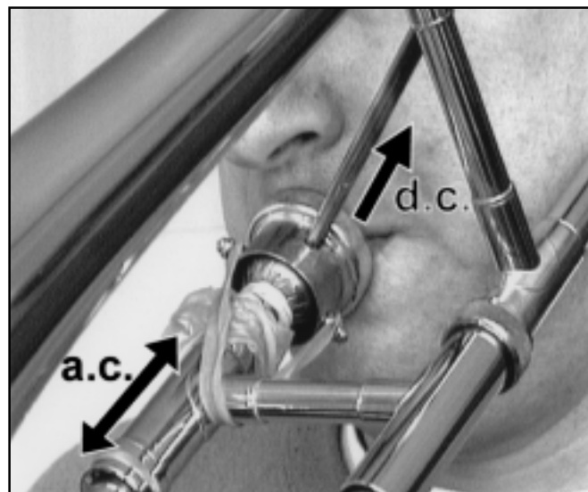
Figure 5. The modified mouthpiece in use with a trombone. This size instrument was chosen to make working with diaphragms and mouthpiece throats easier.
