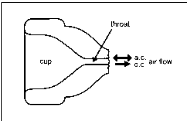
Figure 1. Section through a brass instrument mouthpiece.
